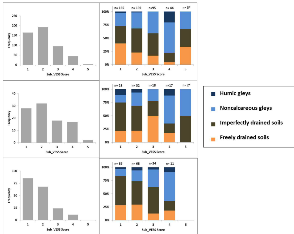
Figure A5:4 - Frequency distribution of the SubVESS scores separated by major soil types after the extreme December/January precipitation for 'In Field' (Top), 'Damaged' (Middle) and 'Margins' (Bottom). SubVESS \leq 2 indicates good subsoil structural condition, whereas \geq 4 indicates severe degradation. Imperfectly and freely drained soils includes Podzols and Brown earths.
