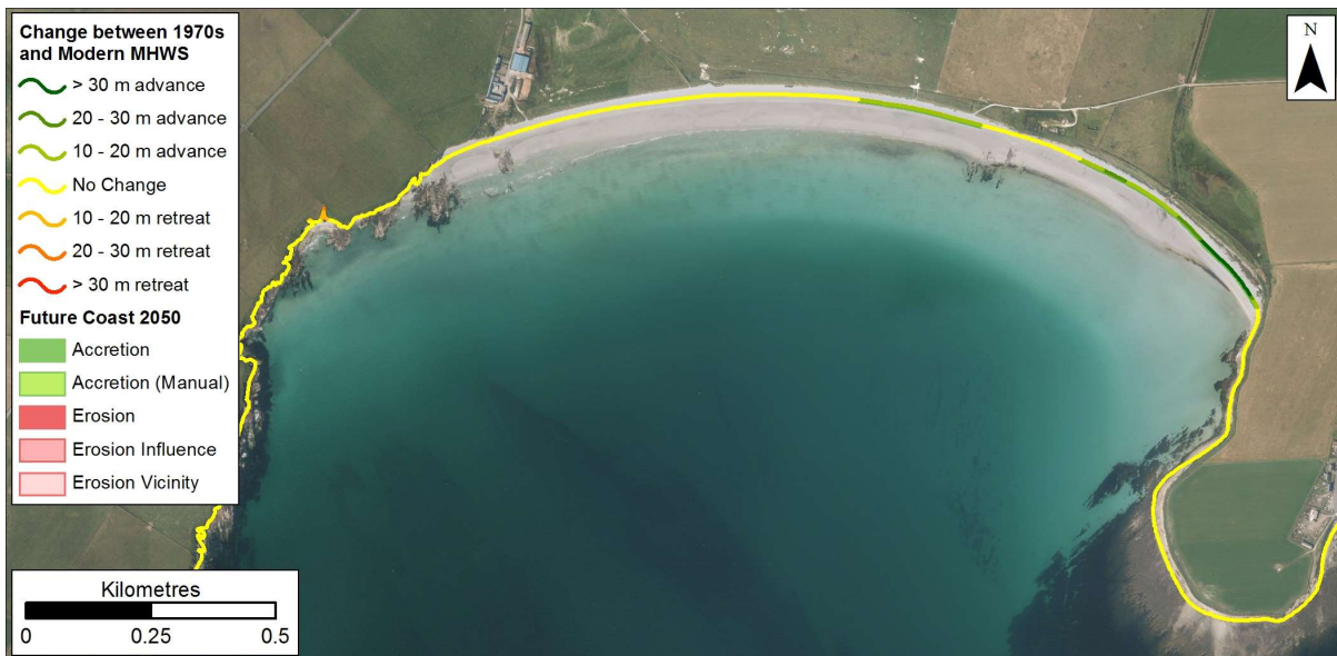
Figure 10.38: Possible future coastline position in 2050 based on rates between 1970 and Modern MHW data at Backaskail Bay. Getmapping are our current providers of Scotland-wide digital aerial imagery© Getmapping plc.
