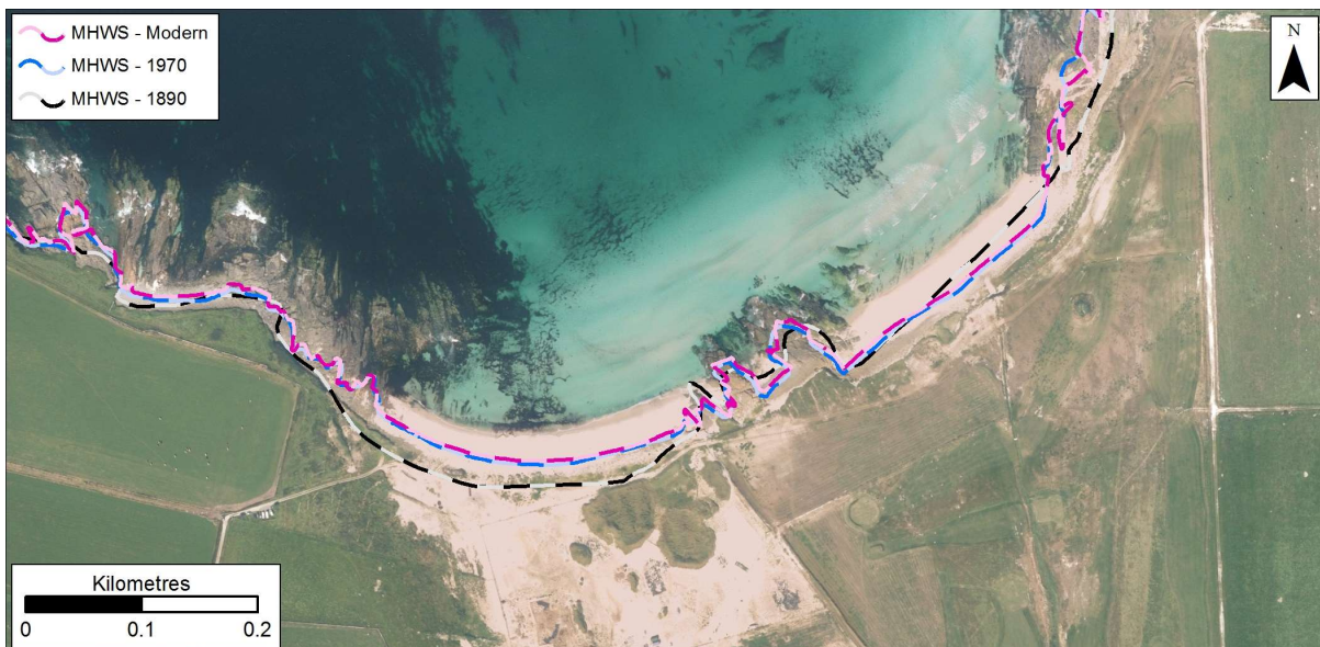
Figure 10.29: MHWS position in 1890, 1970s, and Modern datasets at the Links of Notland. Getmapping are our current providers of Scotland-wide digital aerial imagery© Getmapping plc.
