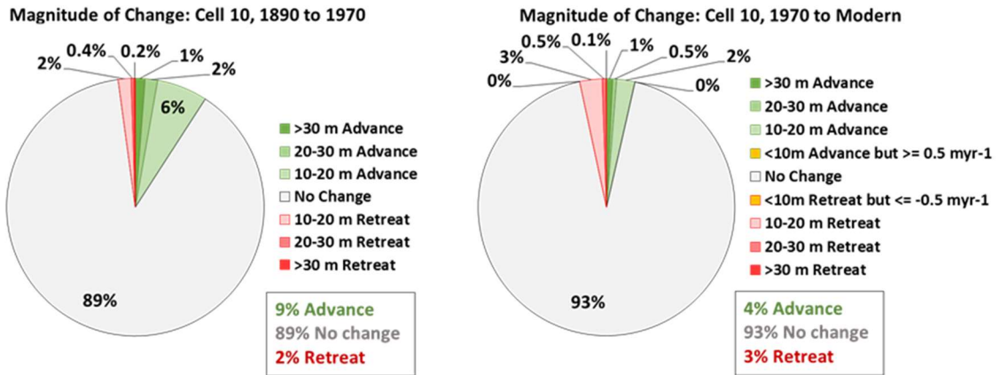
Figure 10.2: Coastal change results for Cell 10 showing the proportional amount of change in the historical (ca. 1890-1970 normalised) and recent (ca. 1970-Present) periods. Rounding errors may produce small % differences between Figure 2 and Figure 10.2.
